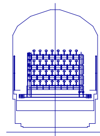
ENLARGED VIEW THROUGH ROLLERBANK (SCALE 1:25)
