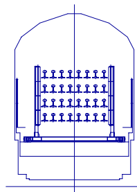
ENLARGED VIEW THROUGH ROLLER-STANCHION (SCALE 1:25)
